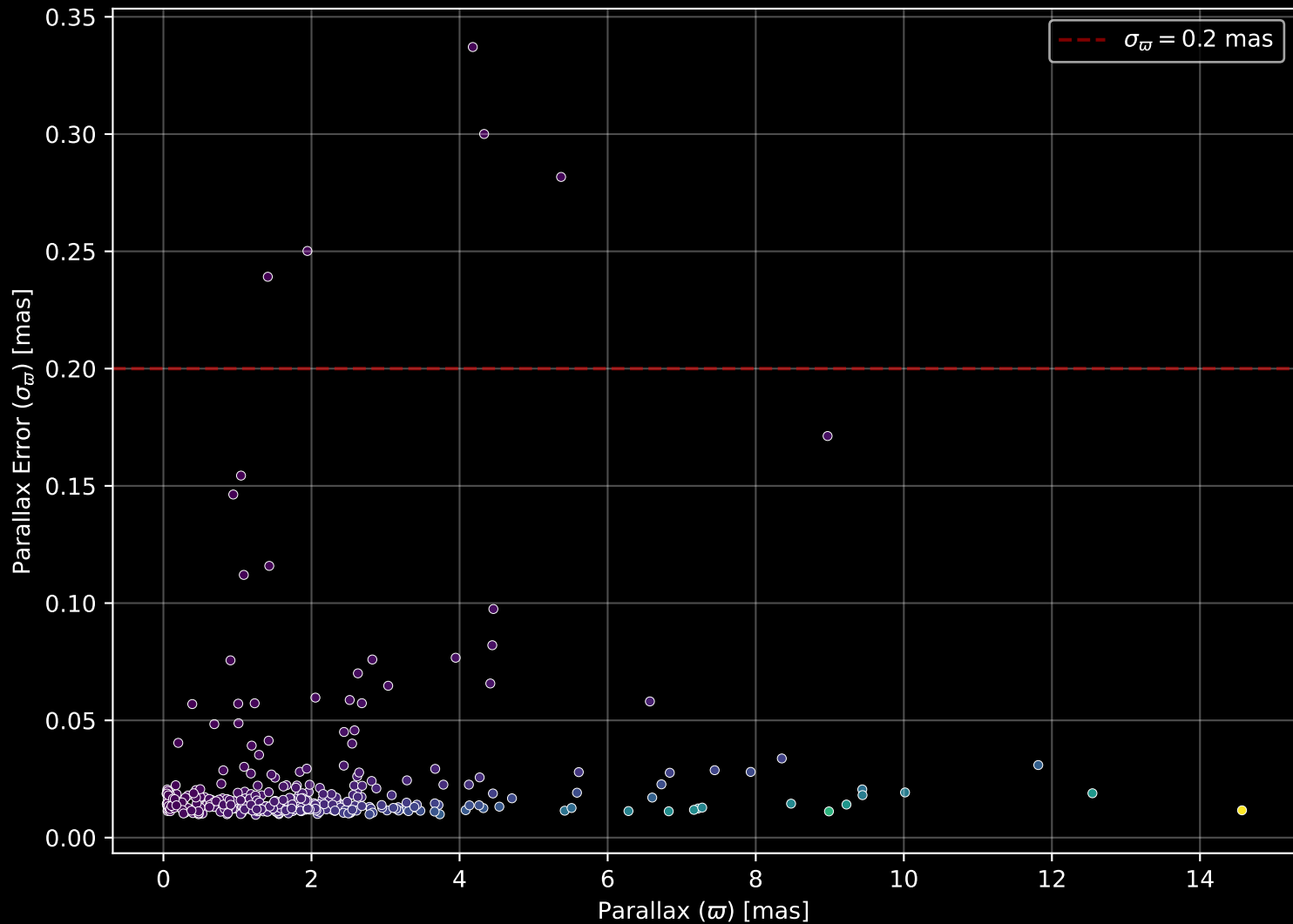
APOGEE DR17 Field: [M79] Parallax Quality (n= 370)
