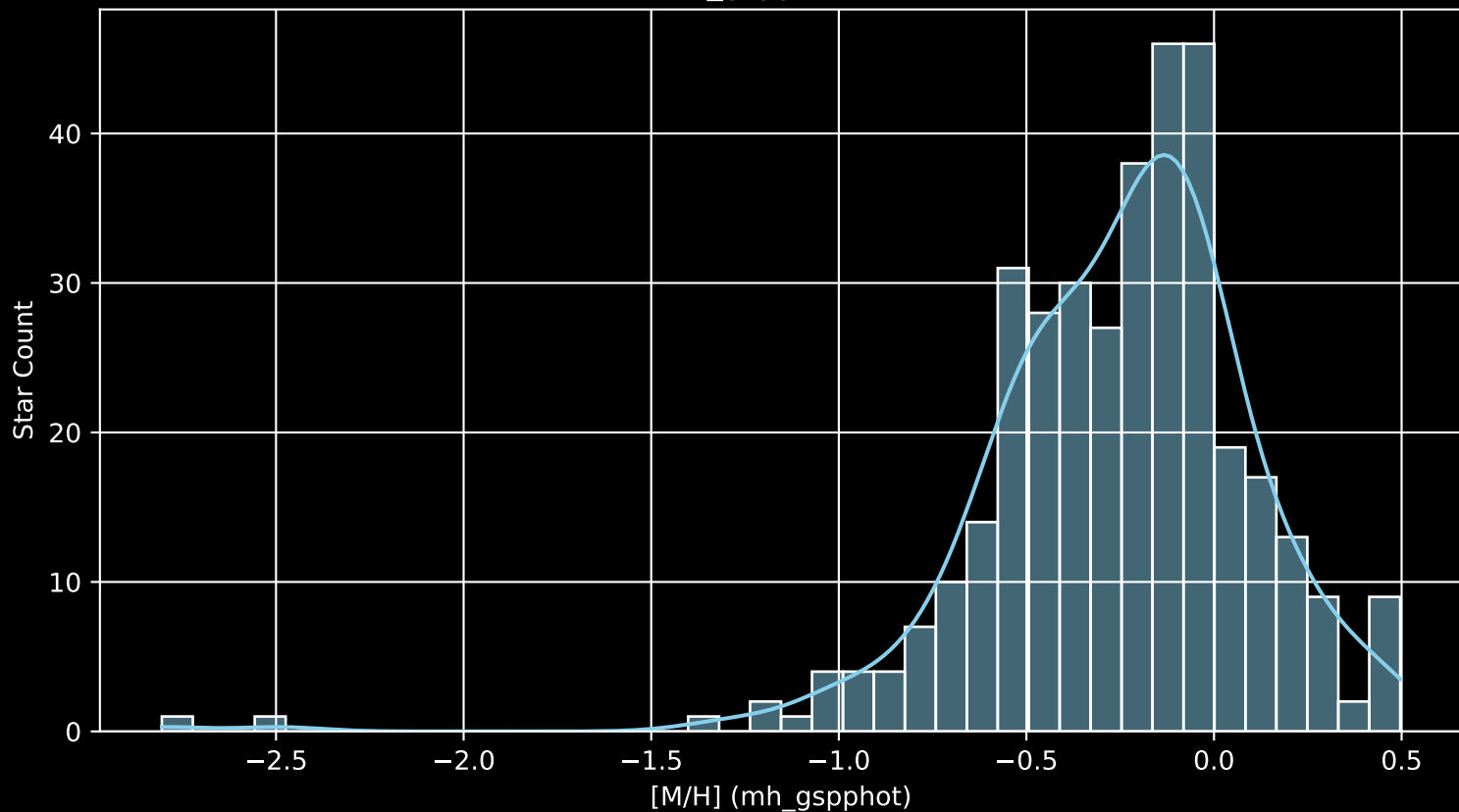
APOGEE DR17 Field: [M79 [M/H] (mh_gspphot) (n= 364)
