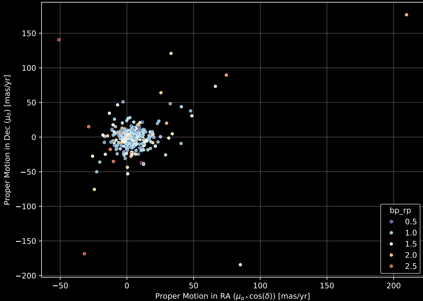
APOGEE DR17 Field: [M79] Proper Motion Diagram (n= 370)
