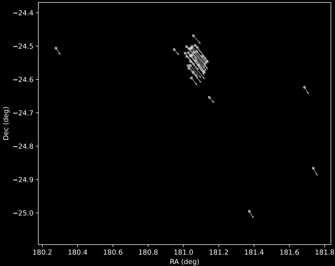
APOGEE DR17 Cluster 15 Proper Motion Vectors (n=31)
