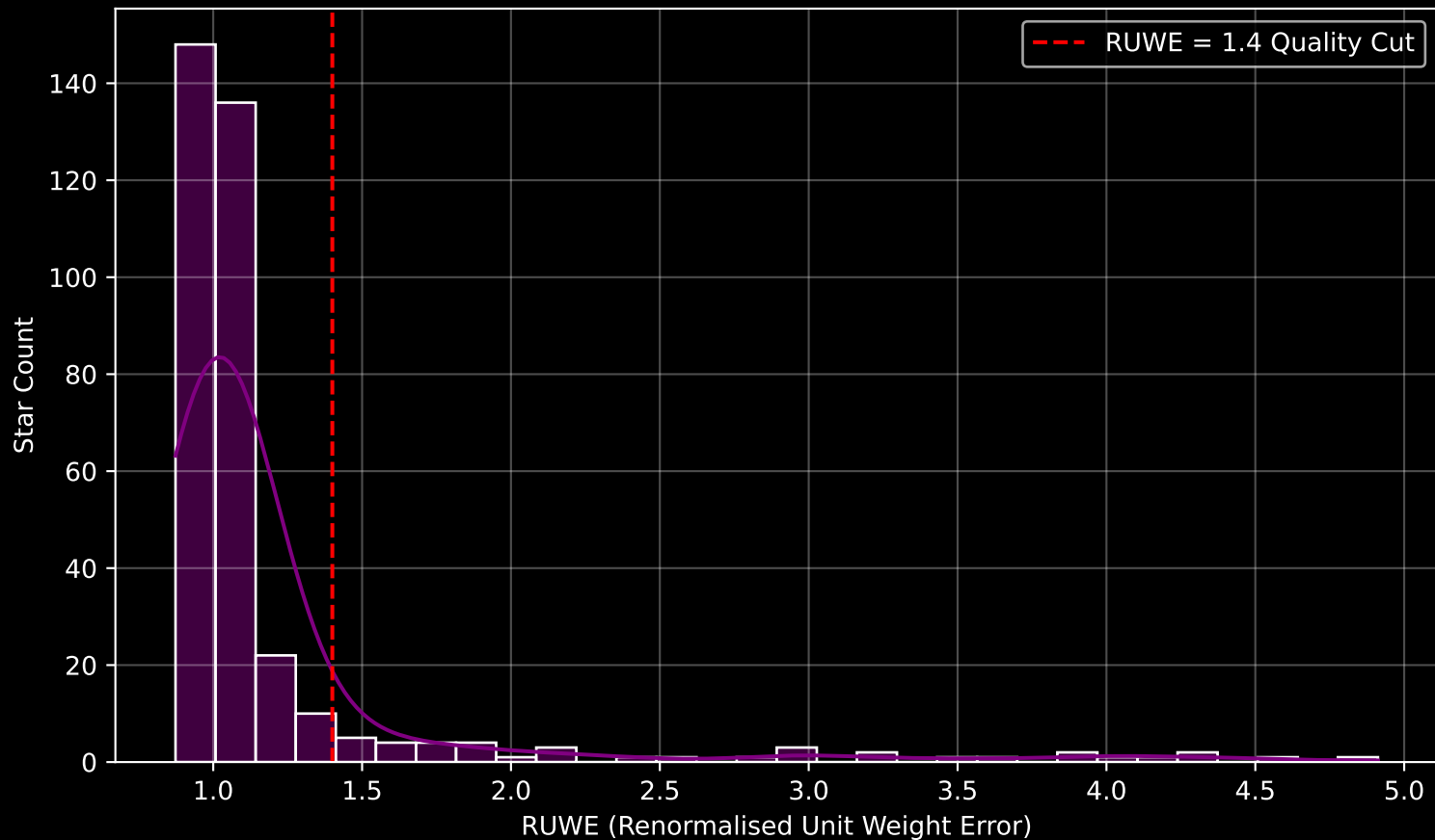
GAPOGEE DR17 Field [M79] RUWE Distribution (n= 355)
