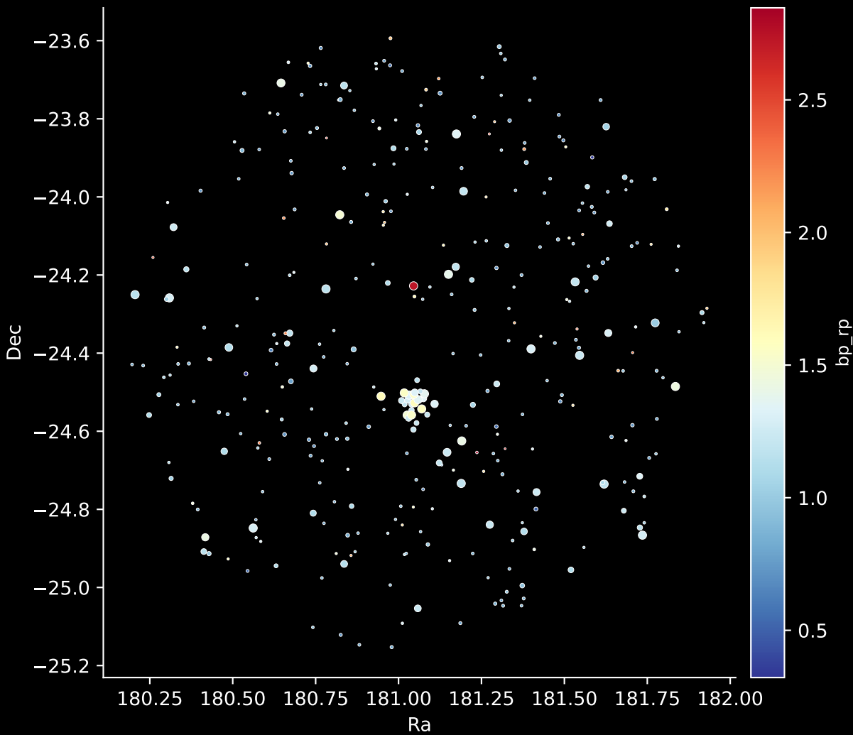
APOGEE DR17 Field: [M79] Stars: 370
