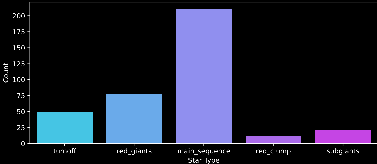
APOGEE DR17 Field: [M79] Count plot of Star Type
