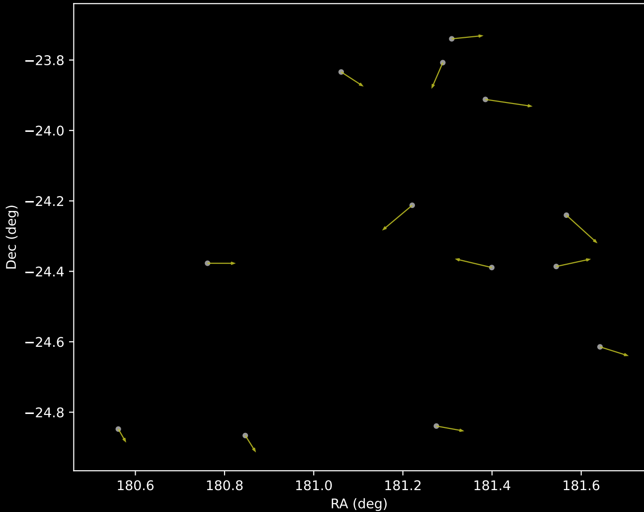
APOGEE DR17 Cluster 16 Proper Motion Vectors (n=13)
